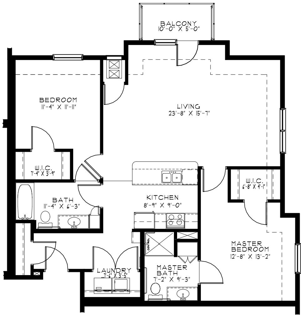
HILLCREST A TYPE "B" 1,208 S.F. 2 BEDROOM (2) TOTAL
