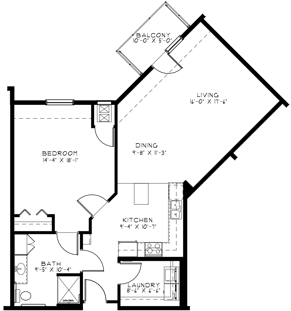
BROWNSTONE TYPE "B" 956 SF 1 BEDROOM (1) TOTAL
