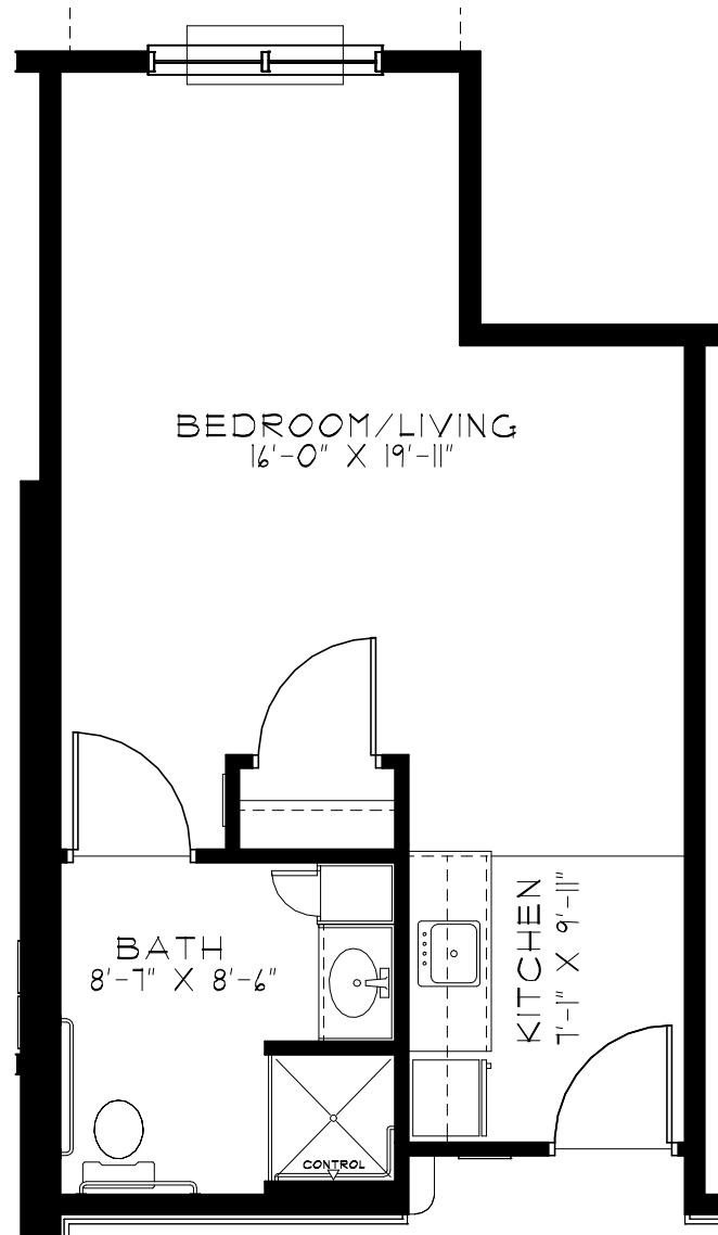
LEGACY J TYPE "B" 438 S.F. STUDIO (1) TOTAL
